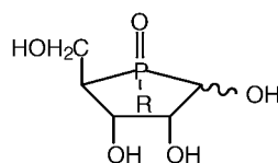
An example of pentofuranose phospho analog, phospho D-ribofuranose
