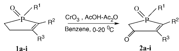
SCHEME 2 Preparation of 4-oxo-2-phospholene 1-oxides 2a-i .
