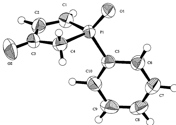
FIGURE 1 ORTEP drawing of compound 2a .
